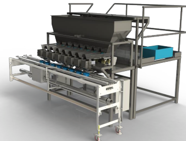
Batch Weighing
